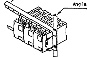
Fig.1 Rack Mounting Panel (FRK-16)
